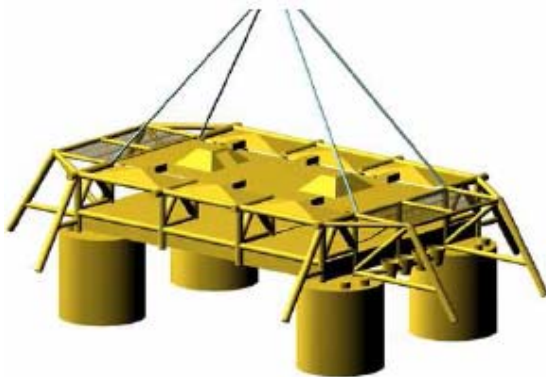
Figure 4. A subsea template
