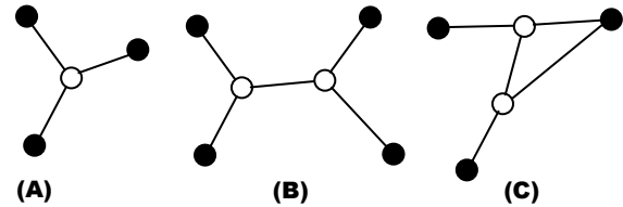
Figure 2. Position uniqueness conditions: (A) One hop multilateration (B) and (C) Two hop multilateration
