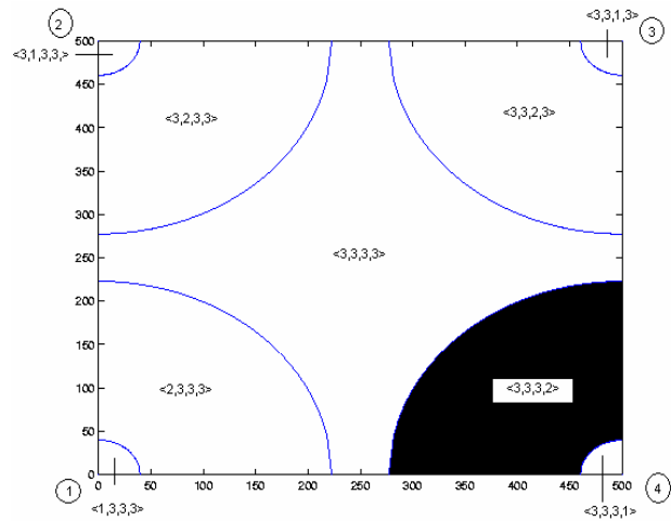
Figure 3. An example of the ALS. Shaded region is \langle 3, 3, 3, 2 \rangle
