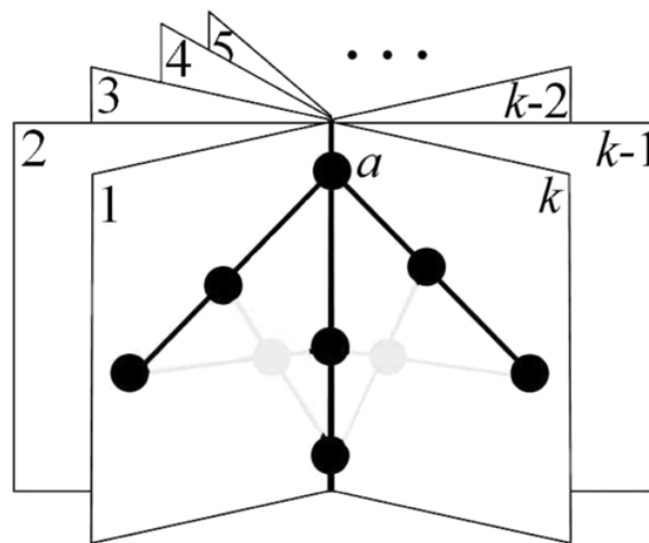
Fig. 8. Geometric representation of M(K_{1,1,k+1}) in rank k + 1 .
