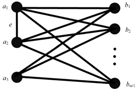
Fig. 9. The graph K_{3,m'-1} .
