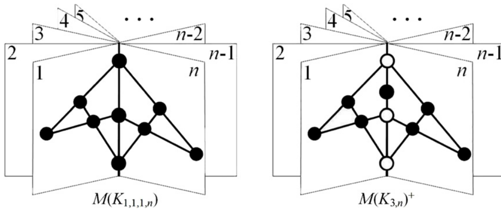
Fig. 7. Geometric representations of M(K_{1,1,1,n}) and M(K_{3,n})^+ .
