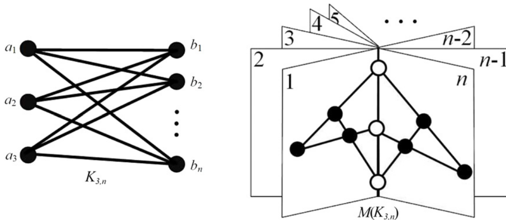
Fig. 6. The graph K_{3,n} and the geometry of M(K_{3,n}) with white dots representing points that are not present in the matroid.
