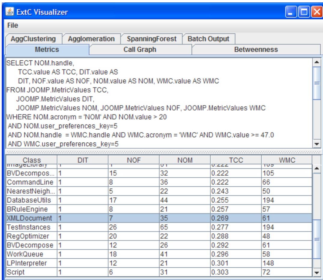
Figure 4.2: ExtC metrics view
