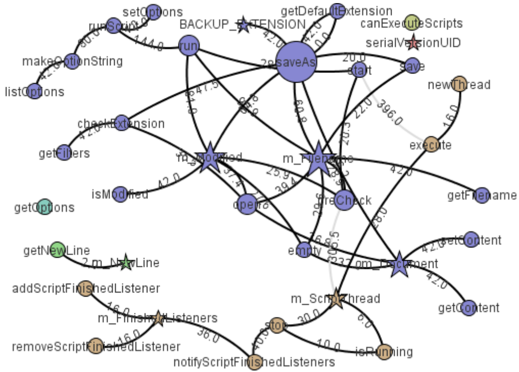
(b) Iteration 2
