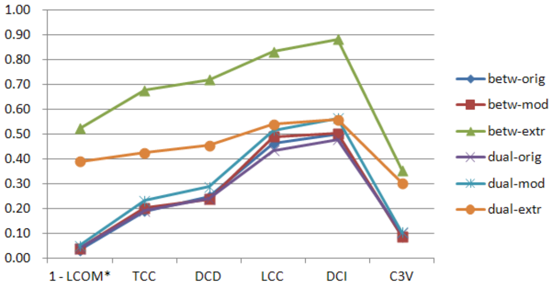
Figure 7.6: Average cohesion values
