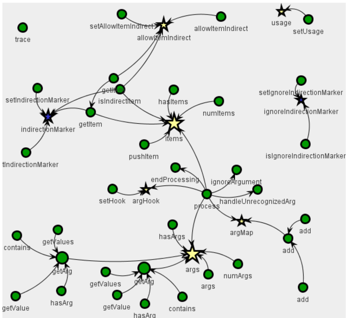
Figure 5.11: CommandLine intraclass dependency graph
