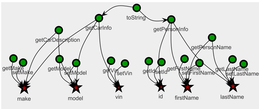
(b) PersonCarDirect
