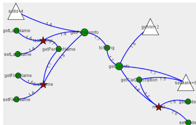
(b) Iteration 6
