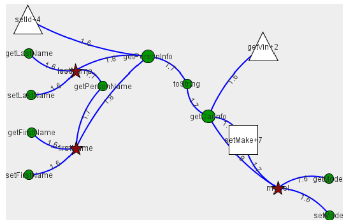
(c) Iteration 7
