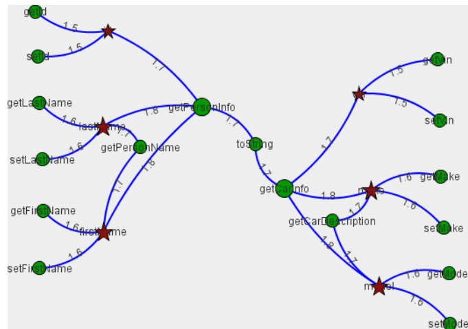
(a) Iteration 0
