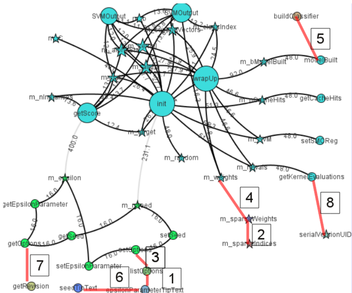
Figure 7.3: RegOptimizer class after dual clustering
