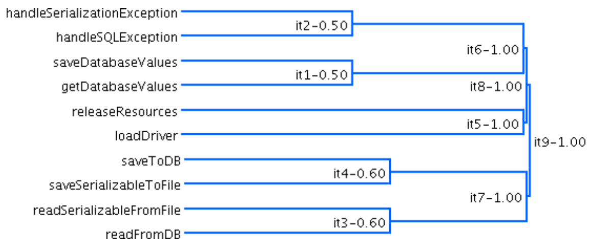
(c) Complete link clustering
