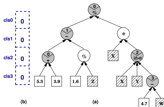
Figure 3. An example Modi program structure. (a) Modi program tree; (b) Output vector.
