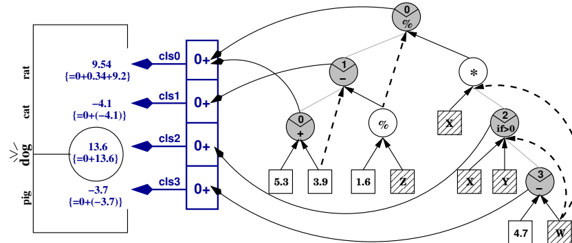
Figure 4. Evaluation of the example Modi program structure.
