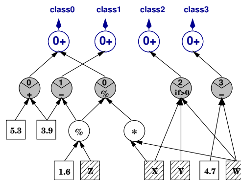
Figure 5. Modi simulated graph/network classifier.
