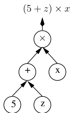
Figure 1. Standard Program Tree (SDtree)
