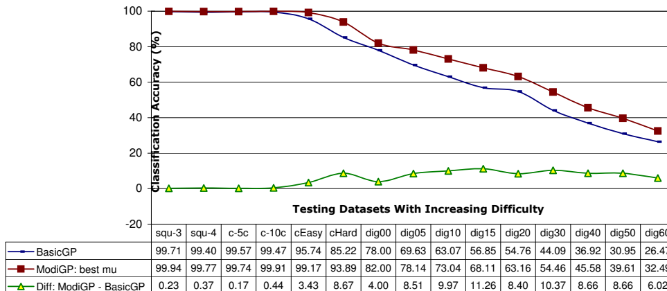
Figure 10. Modi-GP with best and worst modi rates for each classification task.
