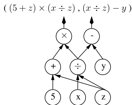
Figure 2. Multiple Roots Program Tree (MRtree)
