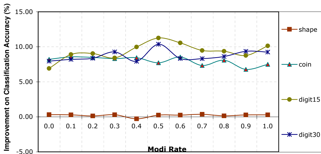
Figure 7. Effect of different Modi rates.
