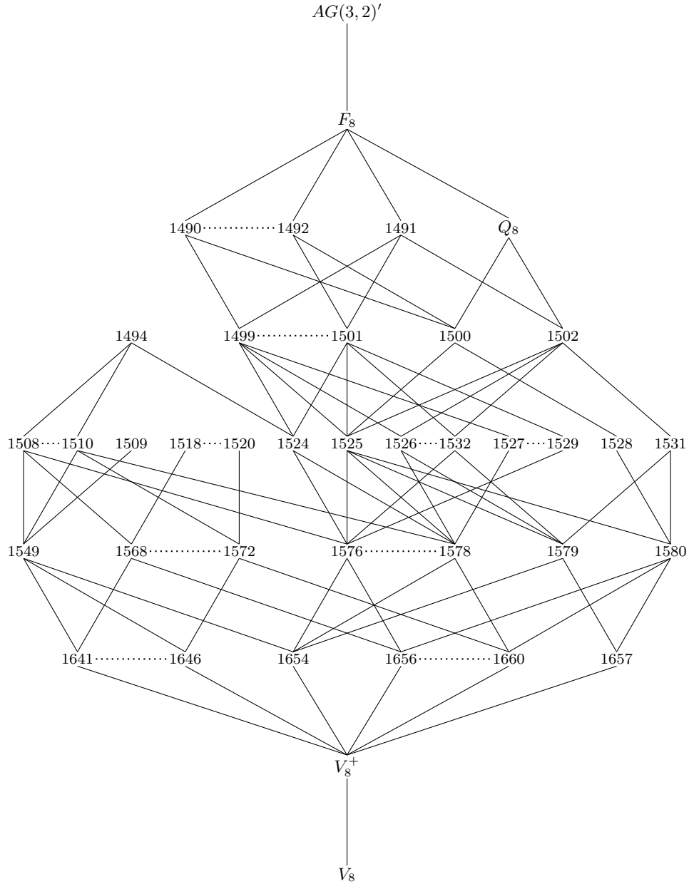
FIGURE 2. The 39 Ingleton-non-representable matroids on 8 elements
