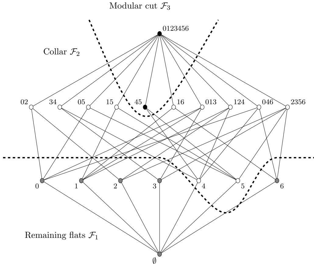
FIGURE 1. A modular cut (black nodes) and its collar (white nodes)
