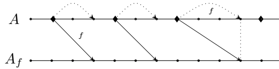
Fig. 2. Construction of sparse and resolute sets.
