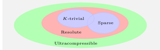
Fig. 1. Classes of sequences of low initial segment complexity.
