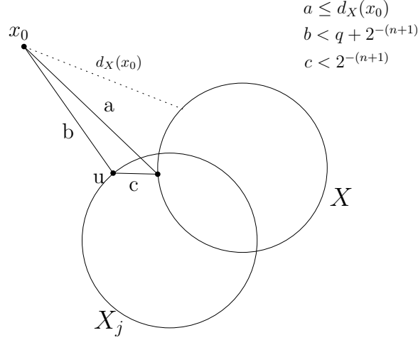
Figure 6: Distances between x_0, u, X, and X_j .
