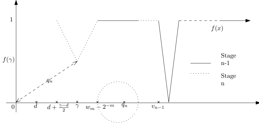
Figure 5: The construction of f if ‘Yes’.
