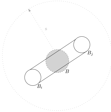
Figure 11: Does B threaten A 's convexity?
