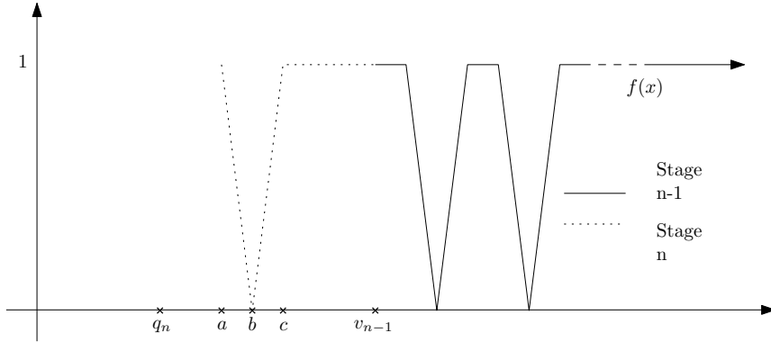
Figure 4: The construction of f if ‘No : I’.
