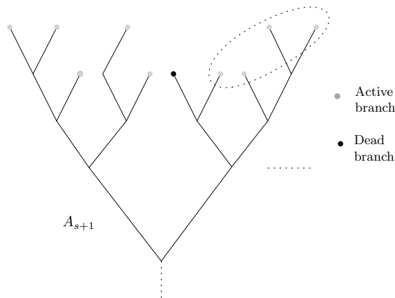
Figure 8: Tree at stage s + 1 .
