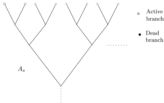
Figure 7: Tree at stage s .
