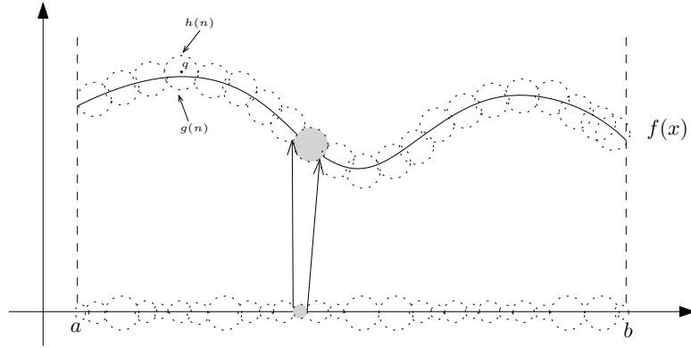
Figure 1: The open ball cover correspondence.
