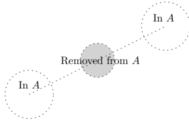
Figure 10: If A not convex.
