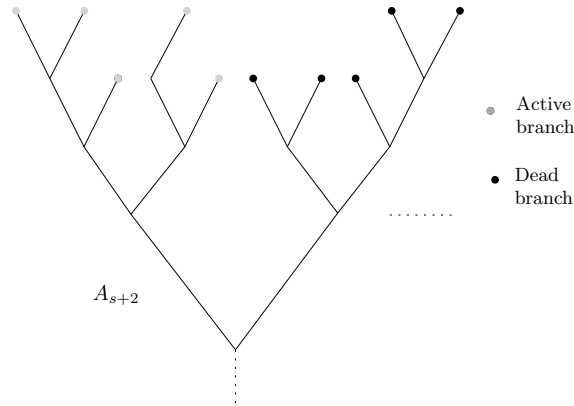
Figure 9: Tree at stage s + 2 .
