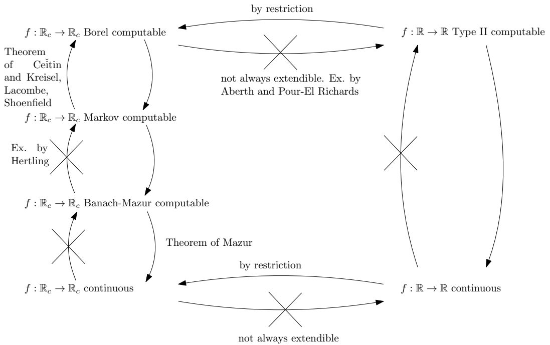
Figure 2: Function relationship summary.
