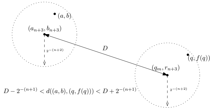
Figure 3: The distance D .
