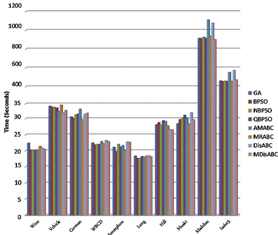
Fig. 2. Average CPU computational times of the algorithms.
