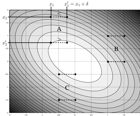
Fig. 1. Detection of interacting variables using differential grouping and CCVIL on different regions of a 2D Schwefel Problem 1.2.
