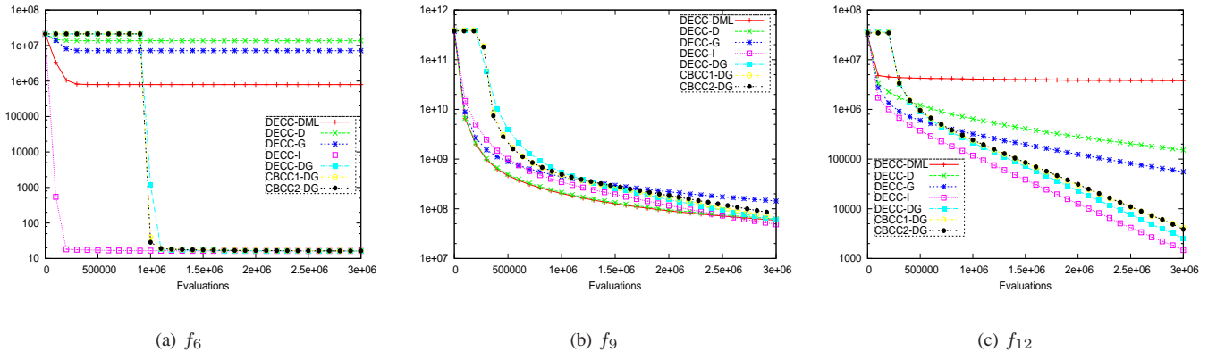
Fig. 2. Convergence plots of various algorithms on selected CEC'2010 benchmark functions. The plots are generated from 25 independent runs.
