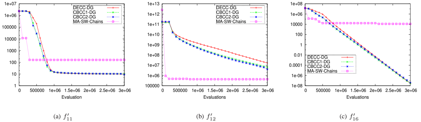
Fig. 3. Convergence of traditional and contribution-based CC using differential grouping against MA-SW-Chains on some representative imbalanced problems.
