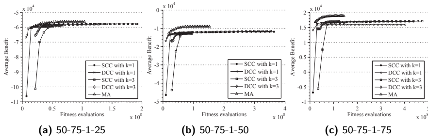
Fig. 6: Convergence curves of the compared algorithms on the TTP instances with n = 50 and m = 75 .
