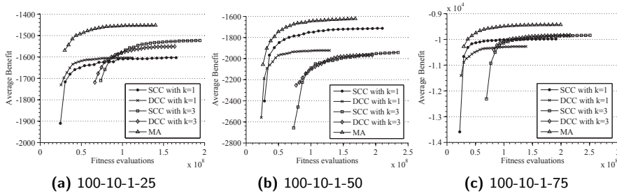
Fig. 7: Convergence curves of the compared algorithms on the TTP instances with n = 100 and m = 10 .
