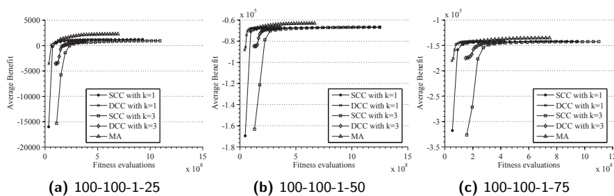
Fig. 8: Convergence curves of the compared algorithms on the TTP instances with n = 100 and m = 100 .
