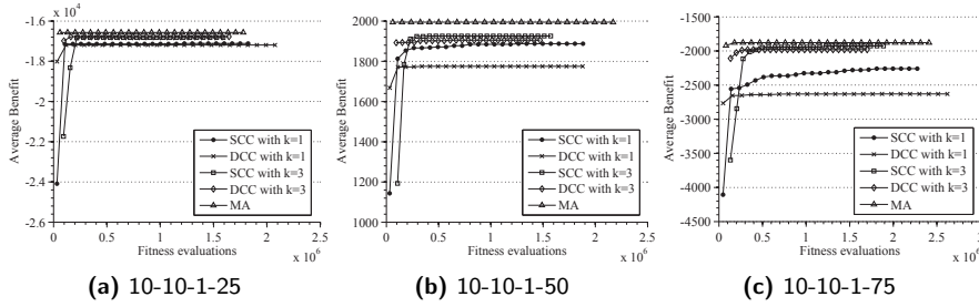
Fig. 2: Convergence curves of the compared algorithms on the TTP instances with n = 10 and m = 10 .
