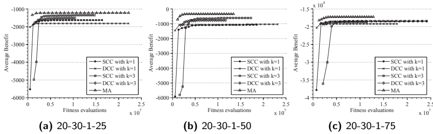
Fig. 4: Convergence curves of the compared algorithms on the TTP instances with n = 20 and m = 30 .
