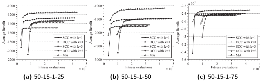
Fig. 5: Convergence curves of the compared algorithms on the TTP instances with n = 50 and m = 15 .
