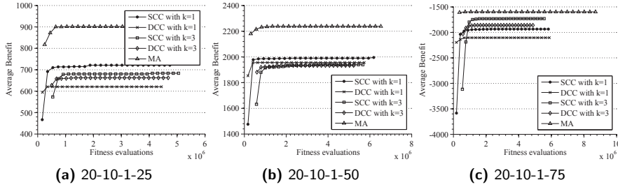
Fig. 3: Convergence curves of the compared algorithms on the TTP instances with n = 20 and m = 10 .
