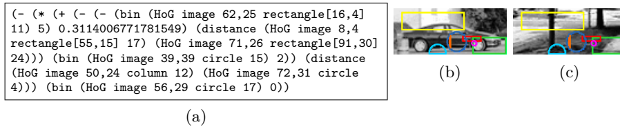
Fig. 5. Example program 3: 96% training and 97% test performance on UIUC dataset (a) Lisp expression, (b) Car (+ve) image, and (c) Background (-ve) image.
