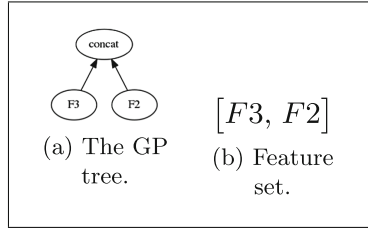
Fig. 3. An evolved vector individual on the Iris dataset (FM: 0.9233).
