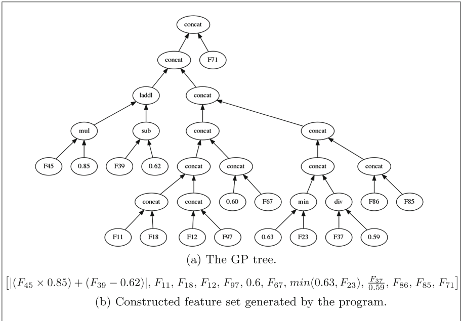
Fig. 2. An evolved vector individual on the 100d40c dataset (FM: 0.499).
