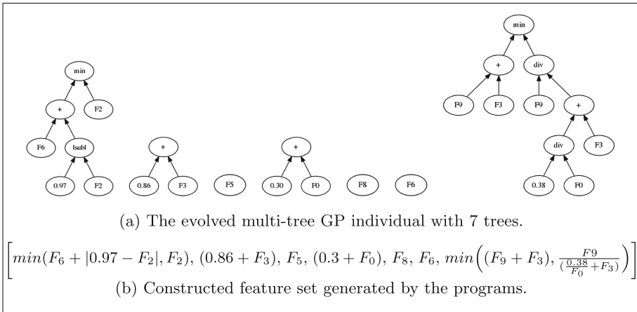
Fig. 1. An evolved multi-tree individual on the 10d20c dataset (FM: 0.9947).
