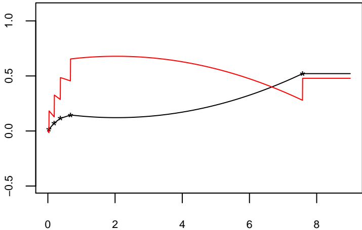
Example of K(x, P_n) and P_n - K(x, P_n)
