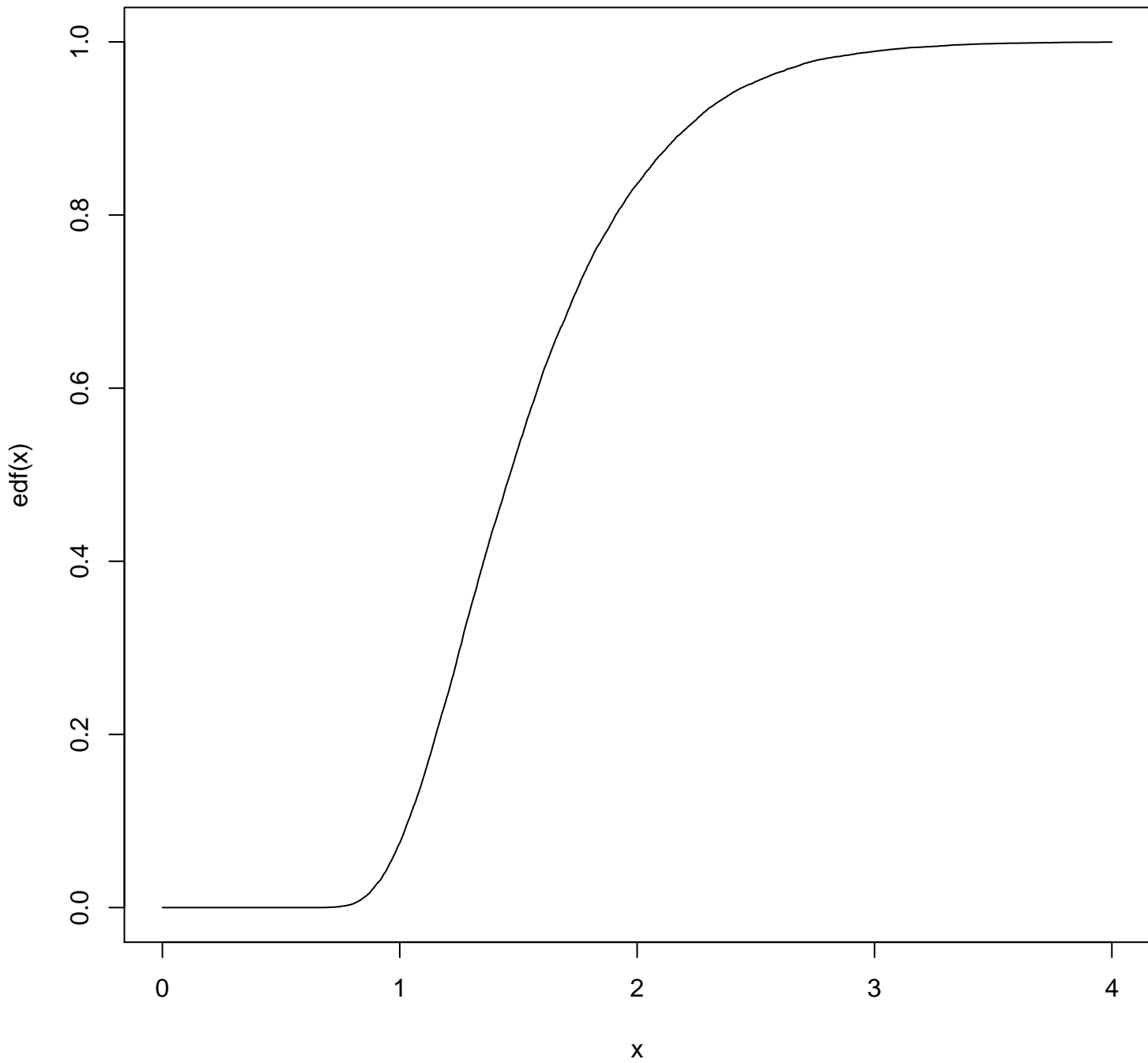
edf for 2D, n=5K, m=20K
