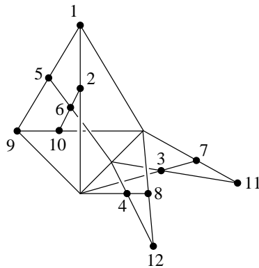
FIGURE 4. A representation of R_{12} .
