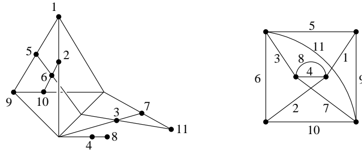
FIGURE 6. R_{12} \setminus \{12\} is cographic.
