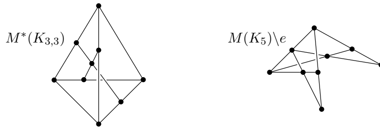
FIGURE 3. M^*(K_{3,3}) and M(K_5)\setminus e .
