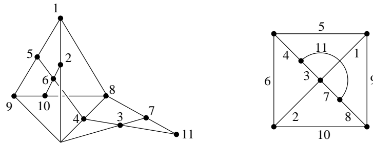
FIGURE 7. R_{12} / \{12\} is cographic.
