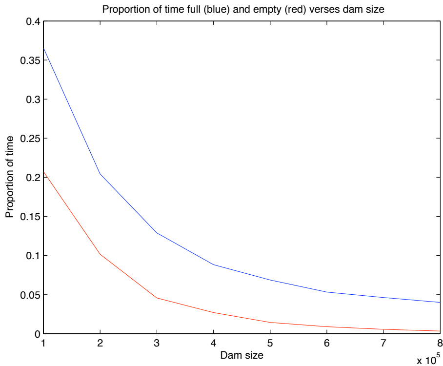
Figure 8.2: Typical proportions of time for empty and overflow conditions as a function of dam size.
