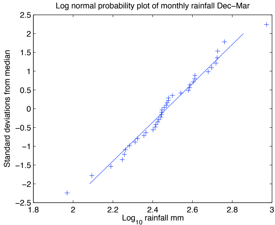
Figure 3.3: Wet season rainfall on a log normal probability plot.
