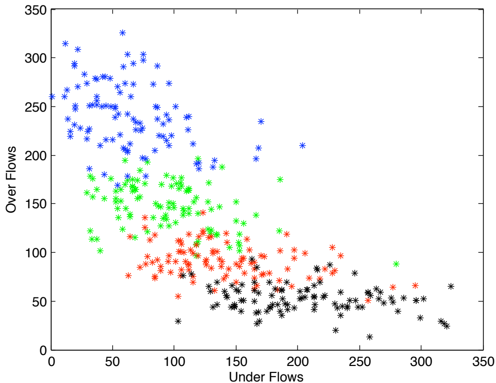
Figure 9.1: Effect of different parameter values for strategy #5 showing the number of months the dam over flows, plotted against the number of months the dam empties (under flows).
