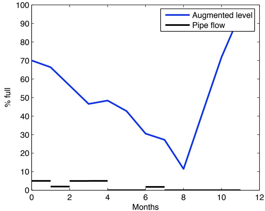
Figure 10.3: Typical progress in water consumption.
