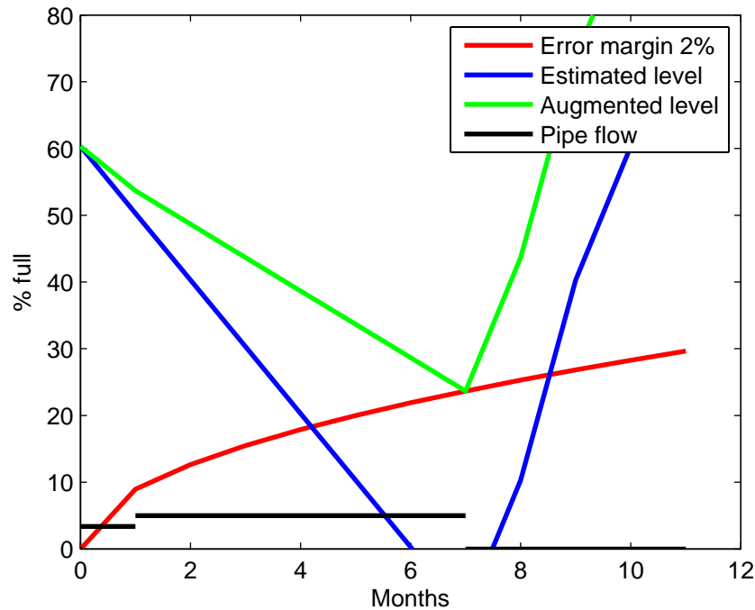
Figure 10.2: Prediction of water requirements after a one month step.
