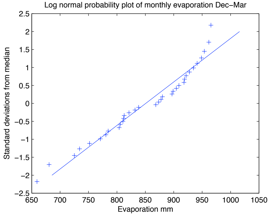
Figure 3.4: Wet season evaporation on a normal probability plot.
