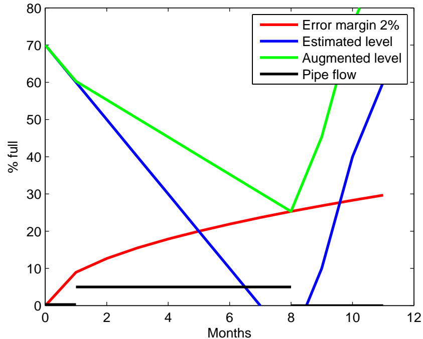
Figure 10.1: Initial prediction of water requirements.
