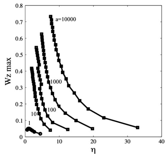
Fig. 13. Simulated values of the maximum rock strain w_z^{\max} , plotted against the similarity variable \eta , one curve for each of a = 10,000, 1000, 100, 10 , and 1 , progressing from right to left through the curves.
