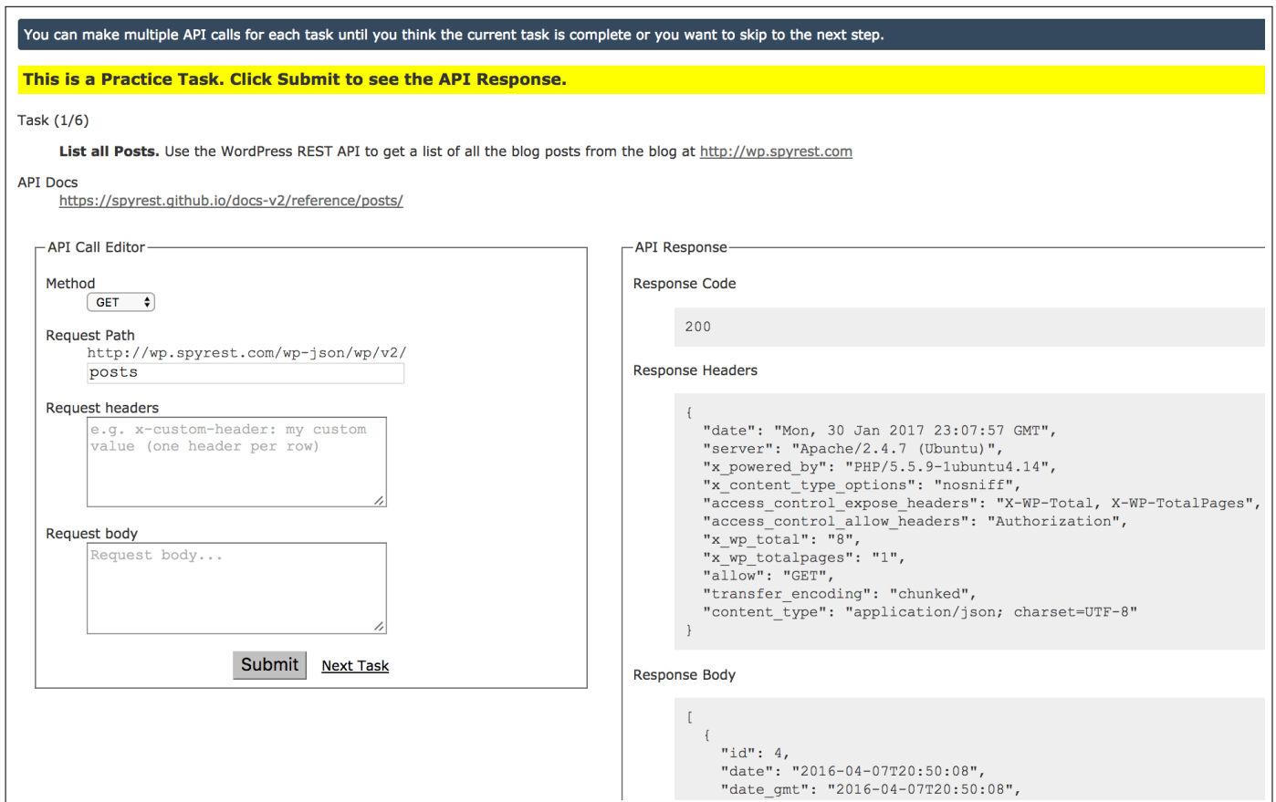
Fig. 2: Screenshot of the Custom-built Web-based REST API Explorer Used by Study Participants
