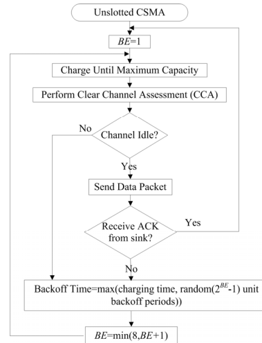
Figure 9. Flowchart illustrating backoff mechanism for unslotted CSMA.
