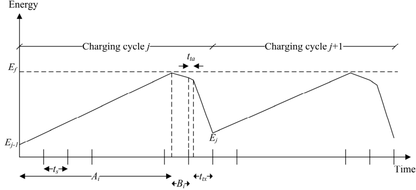
Figure 4. Energy model for slotted CSMA.
