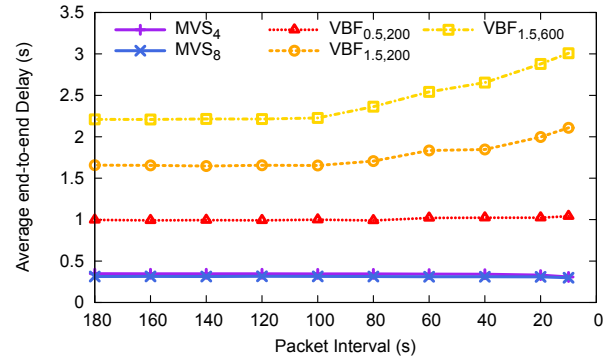
(b) Average End-to-End Delay vs Packet Interval
