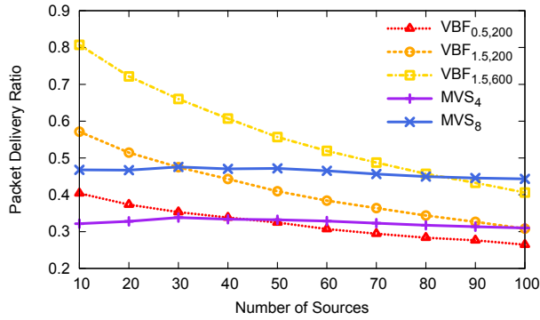
(a) Packet Delivery Ratio vs Number of Sources
