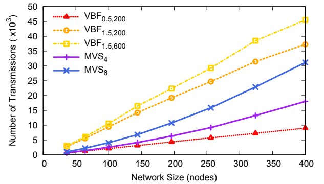
(c) Number of Transmissions vs Network Size
