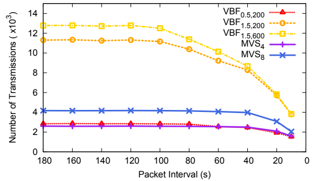
(c) Number of Transmissions vs Packet Interval
