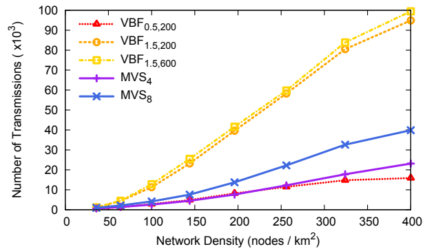
(c) Number of Transmissions vs Network Density
