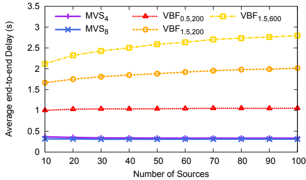
(b) Average End-to-End Delay vs Number of Sources
