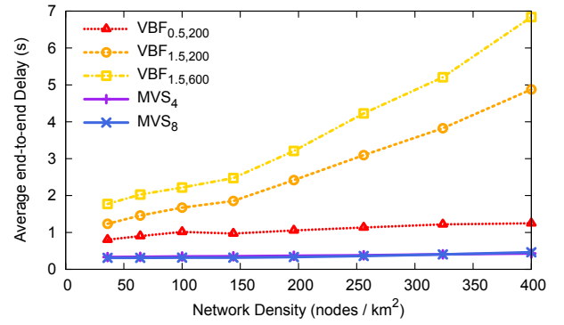
(b) Average End-to-End Delay vs Network Density
