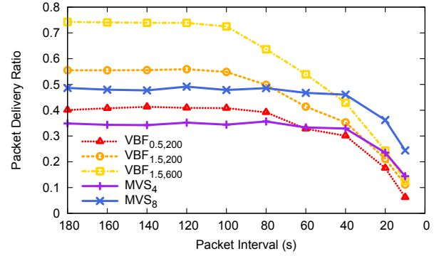
(a) Packet Delivery Ratio vs Packet Interval
