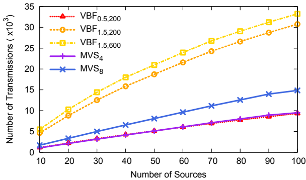
(c) Number of Transmissions vs Number of Sources
