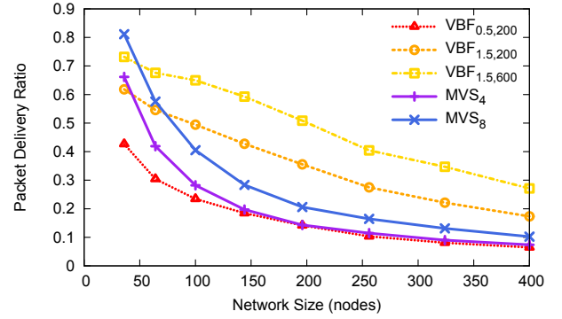
(a) Packet Delivery Ratio vs Network Size
