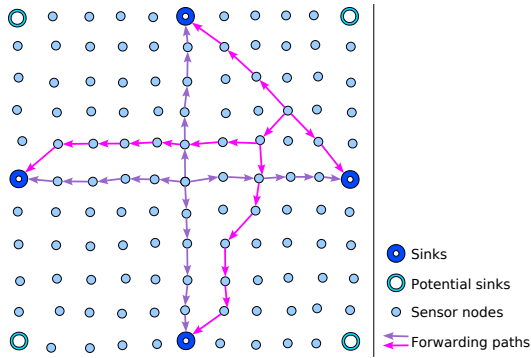
Fig. 1. Multipath Virtual Sink Architecture.
