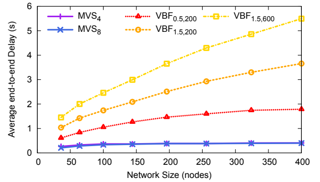
(b) Average End-to-End Delay vs Network Size
