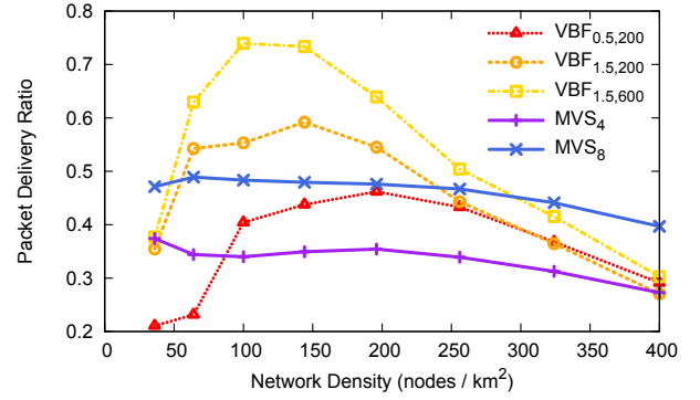
(a) Packet Delivery Ratio vs Network Density
