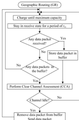
Fig. 7. Flowchart for GR routing protocol
