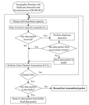
Fig. 9. Flowchart for GR-DD-RT routing protocol
