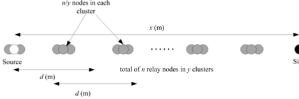
Fig. 6. Cluster String Topology
